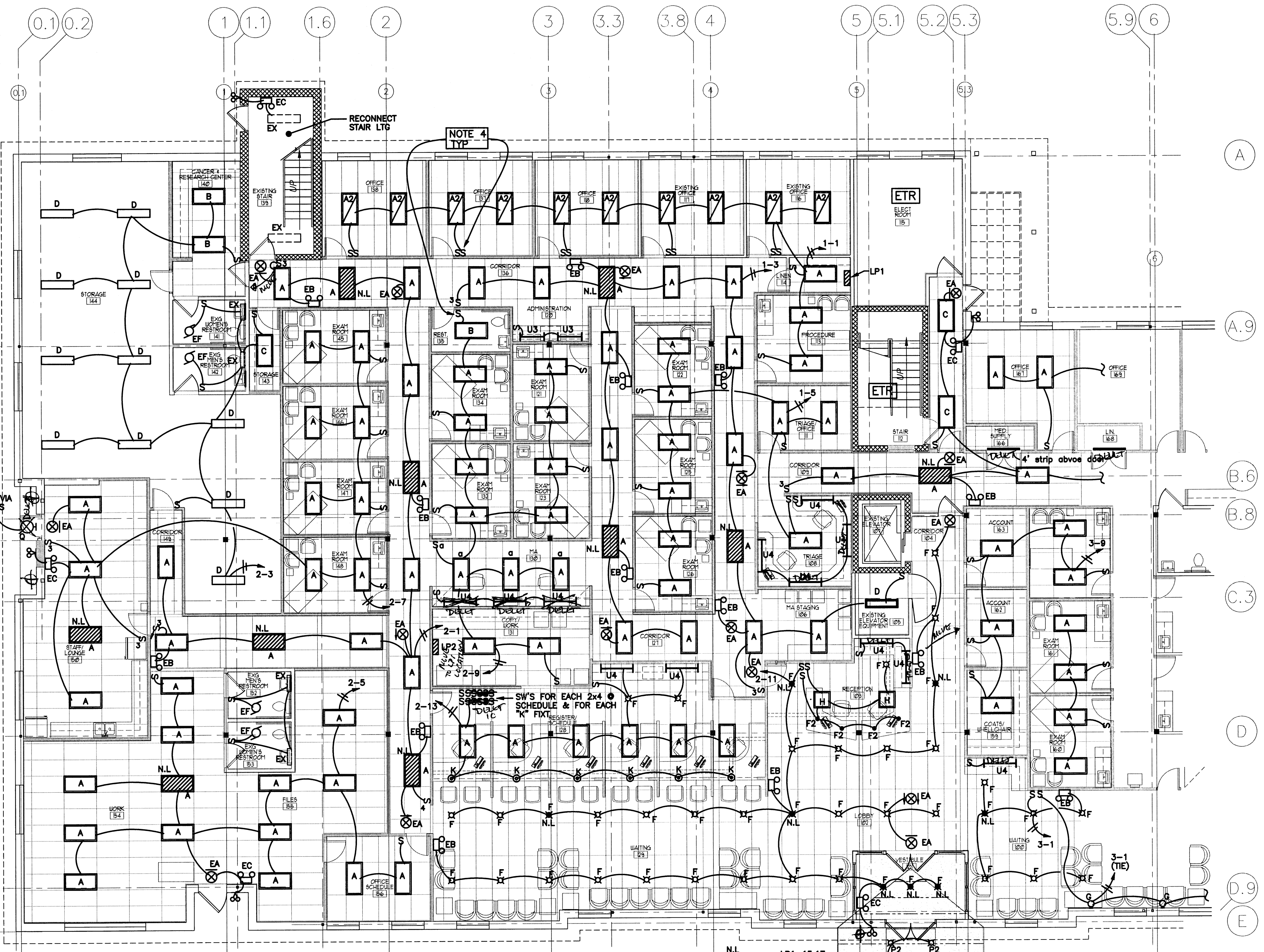
LIGHTING PLAN - WEST SCALE: 1/8"=1'-0"
