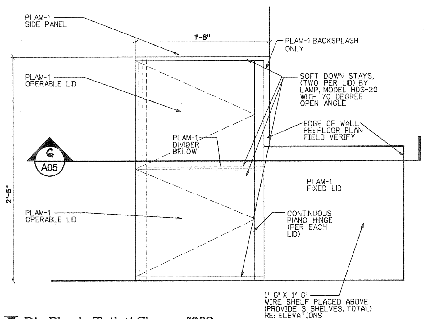
I Bin Plan in Toilet/ Change #208 Scale: 1 1/2"=1'-0"
