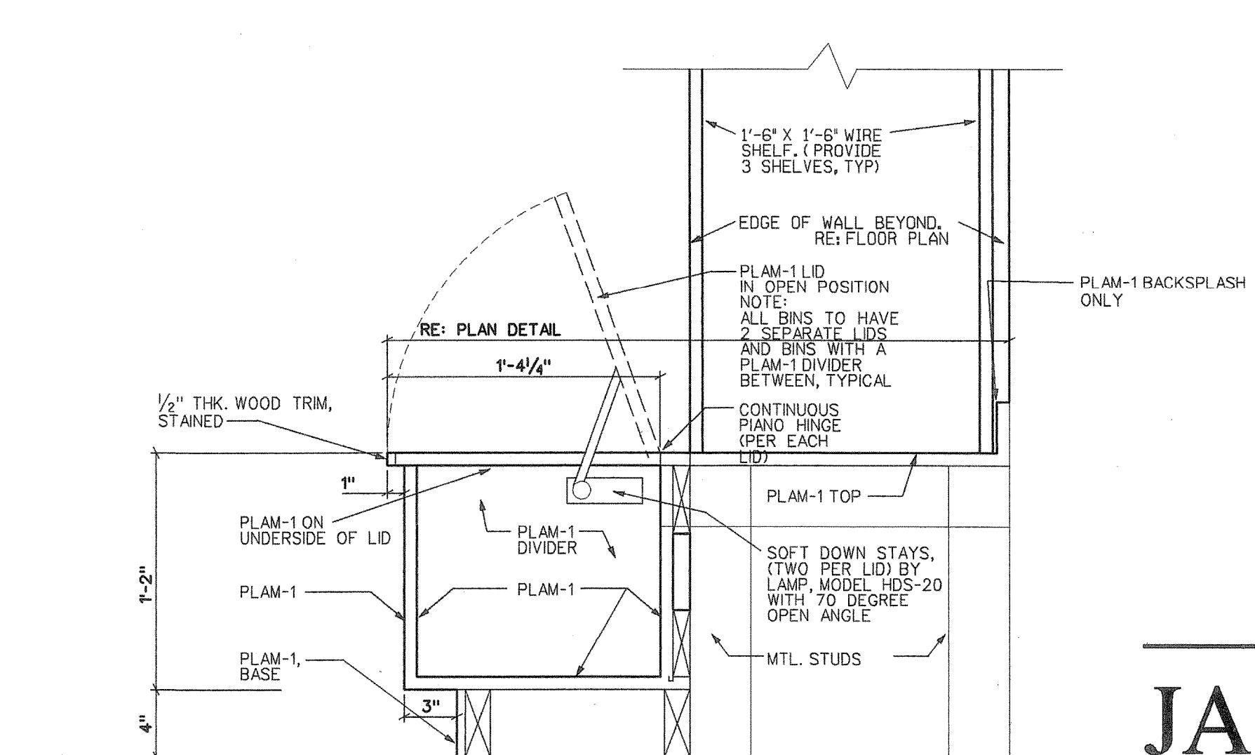
D P-Lam Support Panel Scale: 1 1/2"=1'-0"
