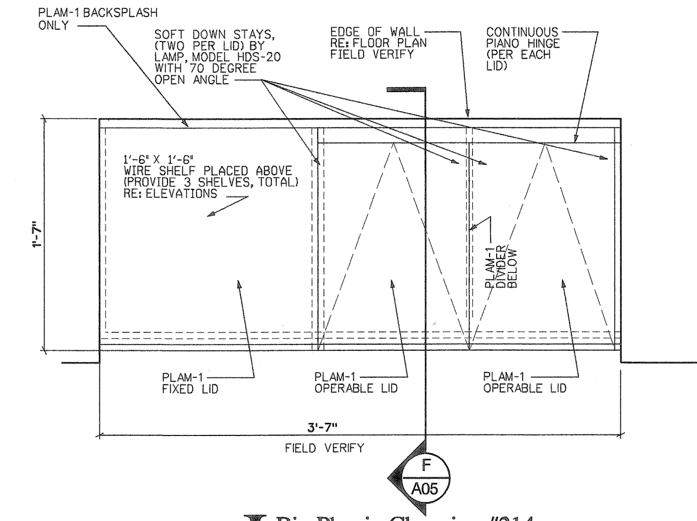
J Bin Plan in Changing #214 Scale: 1 1/2"=1'-0"
