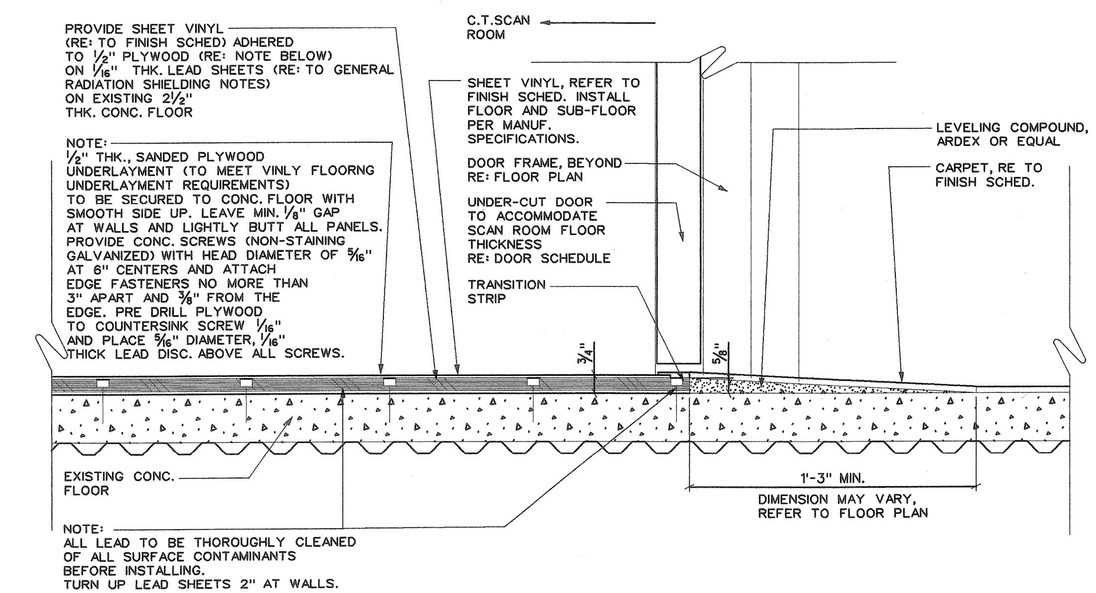
E Lead Floor Detail Scale: 3"=1'-0"
