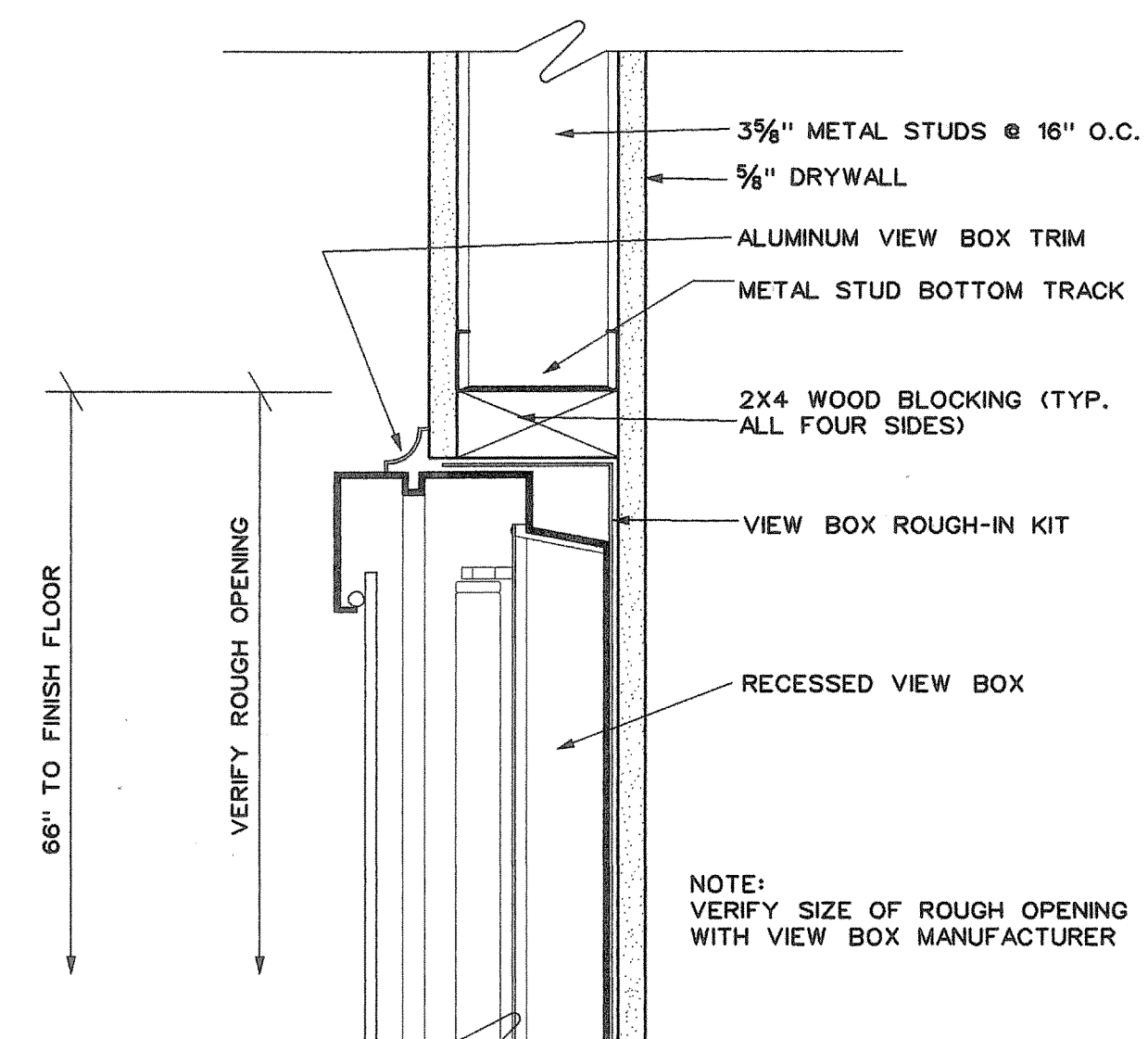
B Recessed X-Ray View Box Detail Scale: 3"=1'-0"
