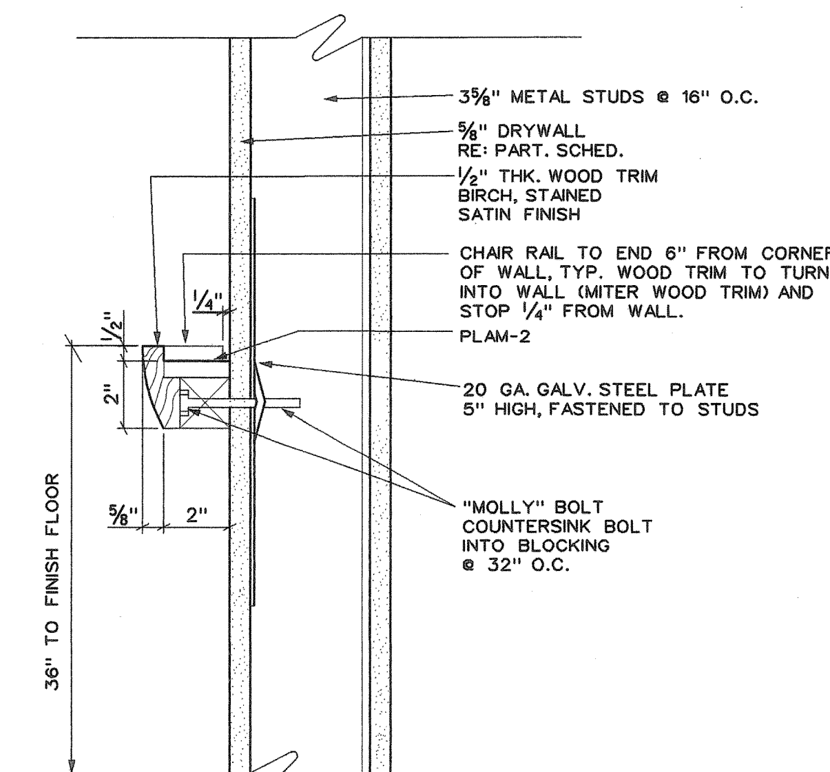
C Chair Rail Detail Scale: 3"=1'-0"
