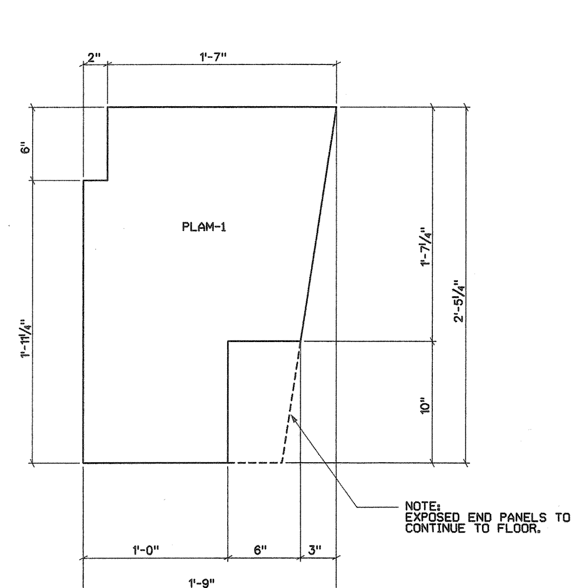
D P-Lam Support Panel Scale: 1 1/2"=1'-0"
