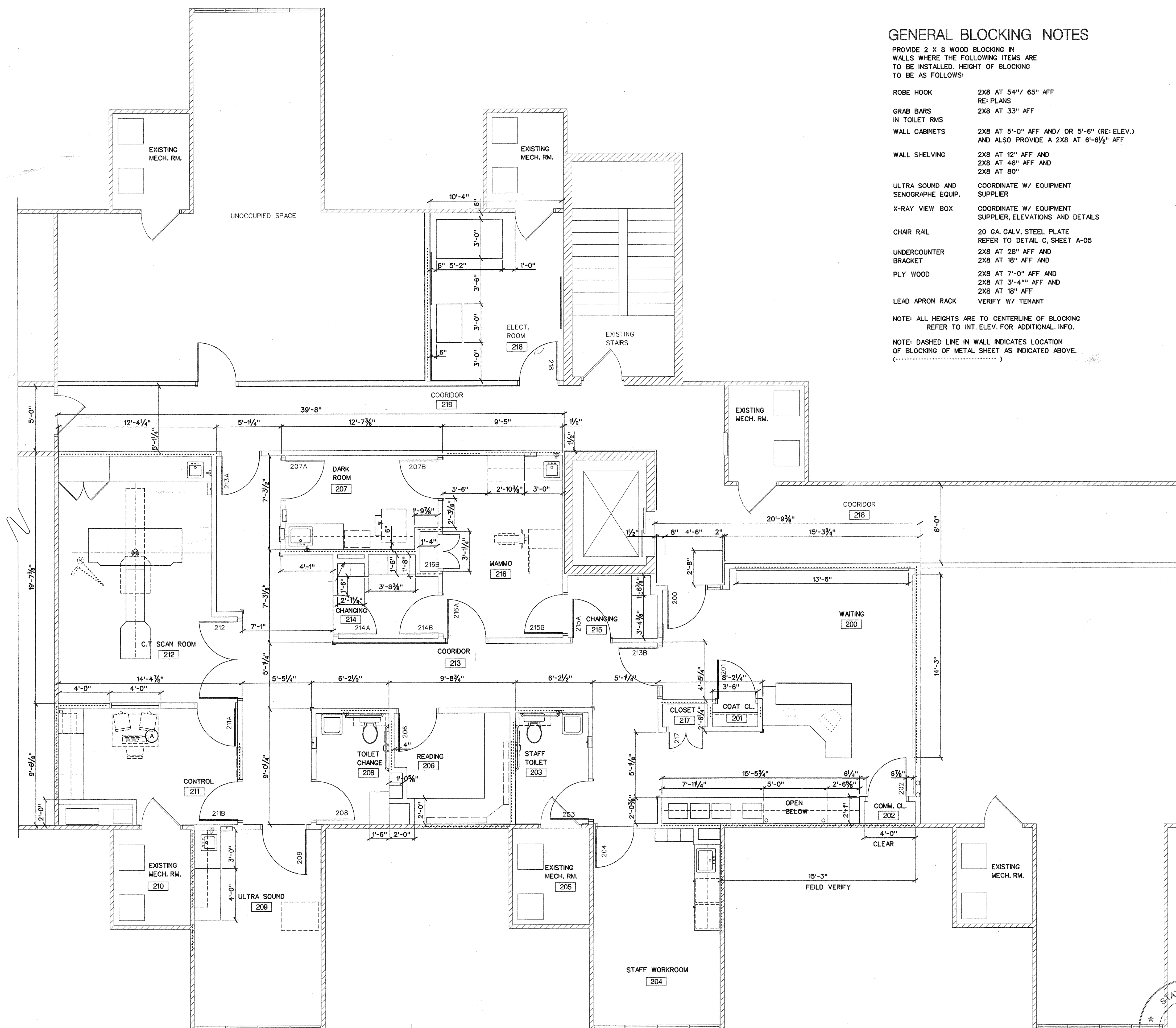
A Second Level Dimension Plan Scale: 1/4"=1'-0"
